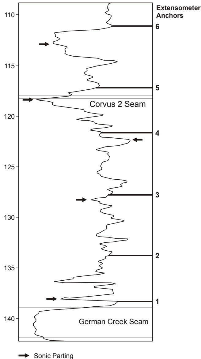
FIG. 3 - Sonic Velocity Log Example
